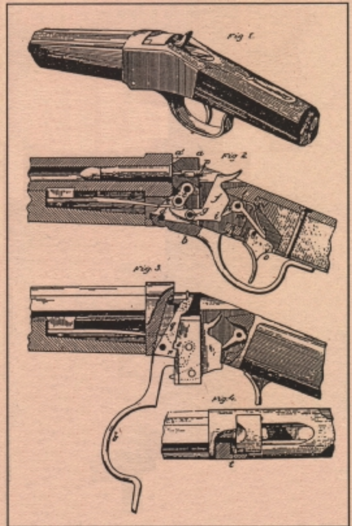
John Browning's first patented arms design for the single-shot rifle.
